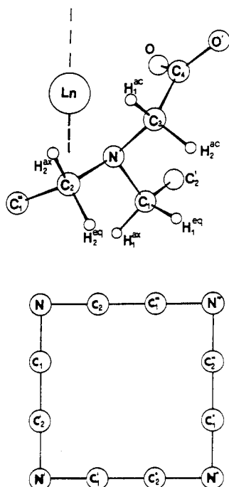
Figure 6. Sketched views of the basic fragment and of the tetraazacyclododecane ring in \text{LnDOTA}^- complexes.
